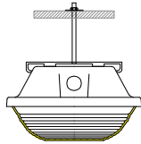
STEM MOUNT
